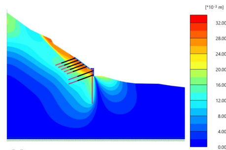
Figure 10 Deformation nephogram of slope during pile-anchor construction
