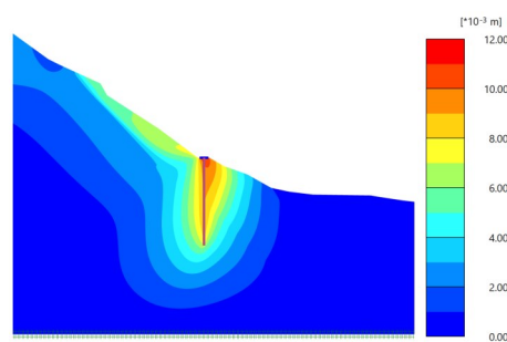
Figure 8 Deformation nephogram of slope during anti-slide pile construction
