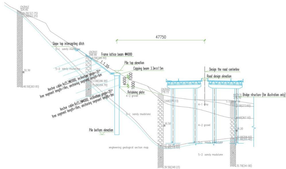
Figure 2 Investigation of the distribution range of landslide accumulation
