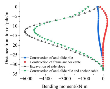
Figure 5 Bending moment diagram of anti-slide piles
