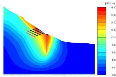
Figure 9 Deformation nephogram of slope during frame anchor cable construction
