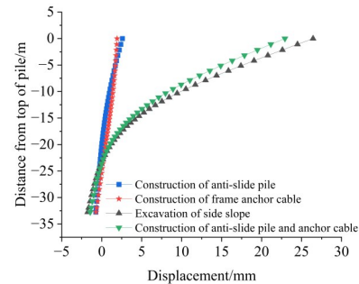
Figure 6 Displacement diagram of anti-slide piles
