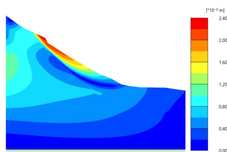
Figure 7 Deformation nephogram of natural slope
