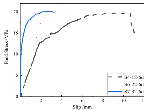
c) Average bond stress–slip curves for S4, S6, and S7
