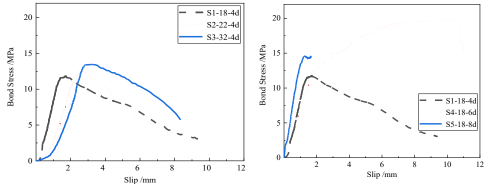
a) Average bond stress–slip curves for S1, S2, and S3
