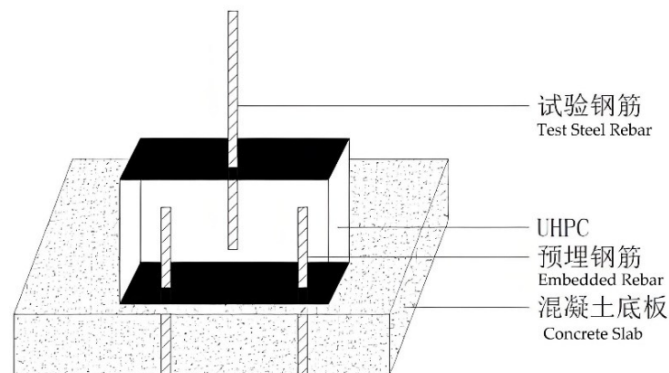
Figure 2 Pull-out test sample design
