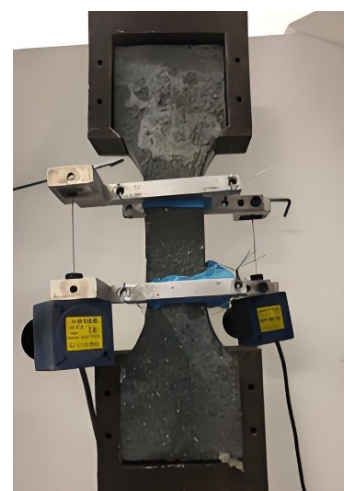
b) Axial tension test setup
