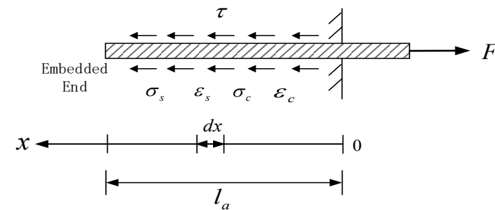
a) Bonded anchoring condition
