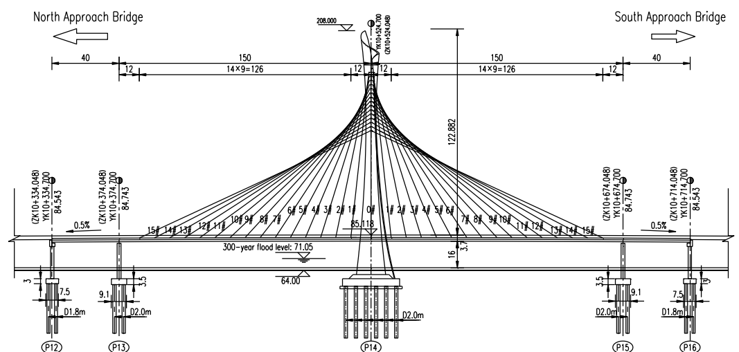
Figure 2 Overall layout of the bridge (Unit: m)
