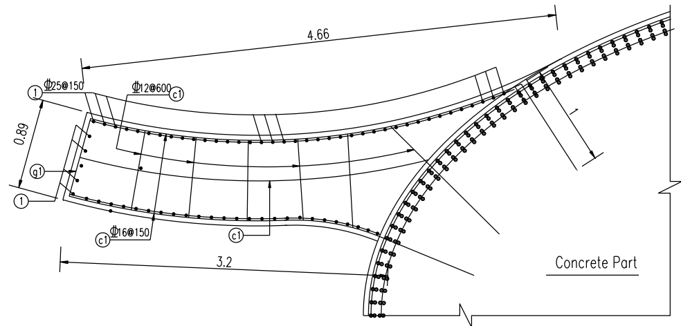
Figure 11 Schematic diagram of the concrete edge rolling structure
