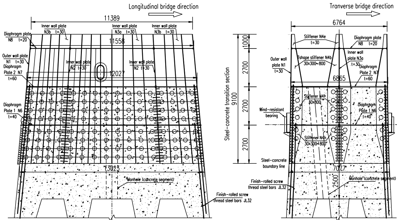
Figure 9 Cross-section / Elevation of the end plate at the steel-concrete transition segment (Unit: mm)
