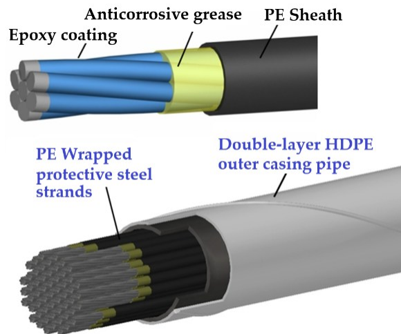
Figure 14 Structural diagram of a steel strand cable
