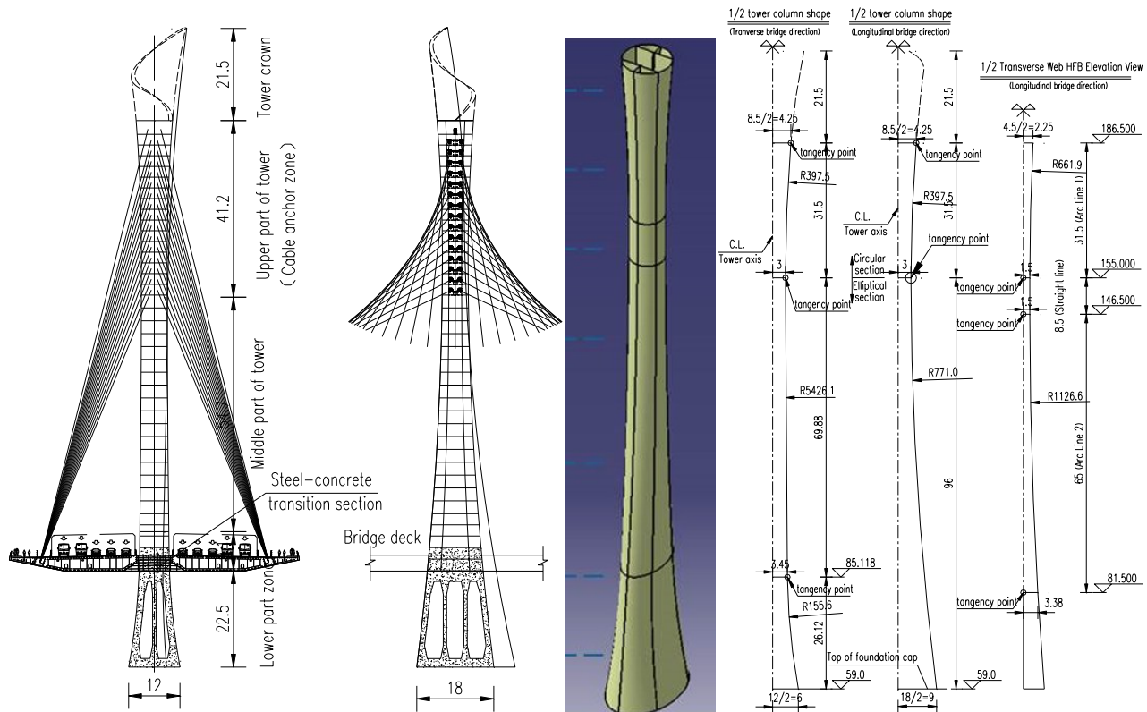
Figure 5 Parameters of bridge tower segmentation and outline (Unit: m)
