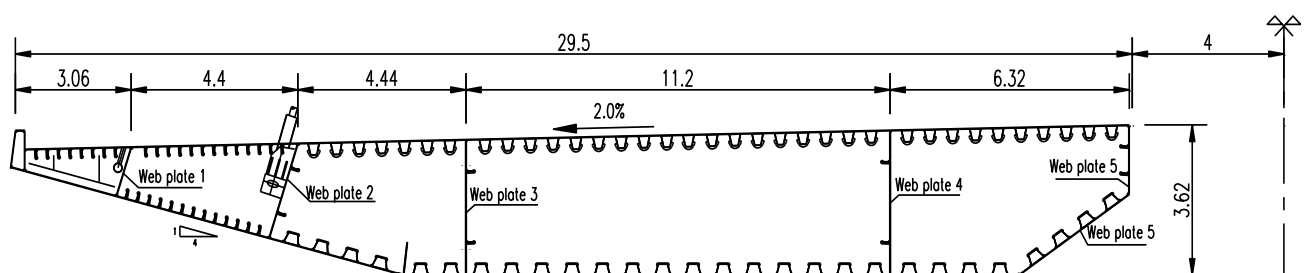
Figure 12 Single-section diagram of the main beam
