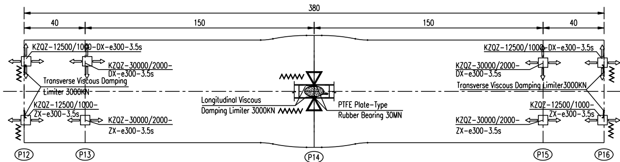
Figure 4 Layout plan of supporting system (Unit: m)
