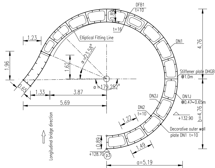
Figure 10 Tower crown section
