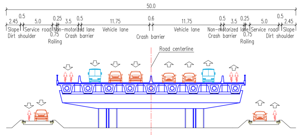
b) Cross-section of the approach bridge
