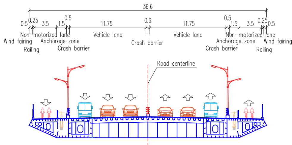
a) Cross-section of the main bridge
