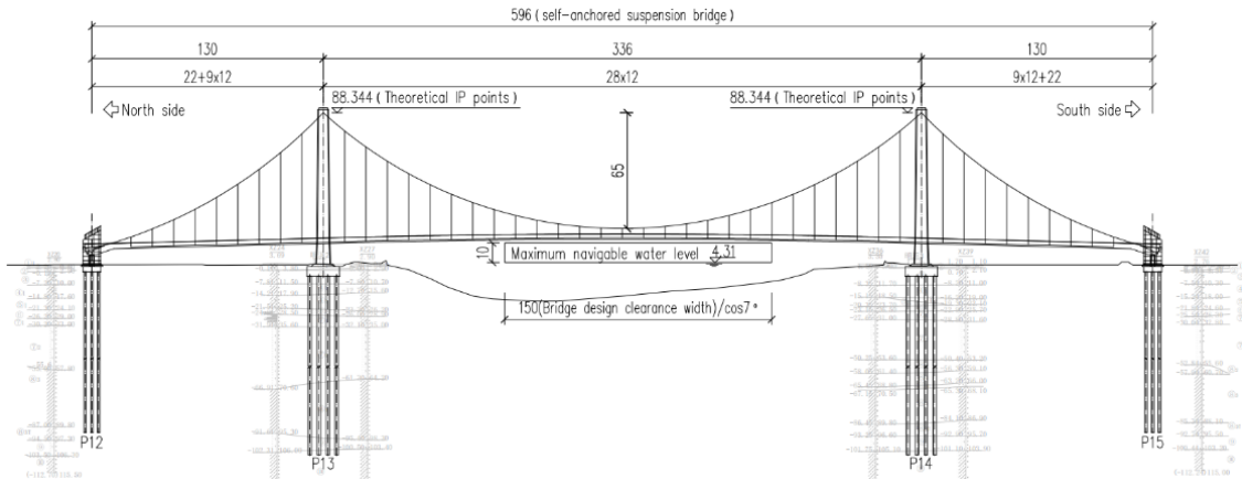
Figure 9 Bridge layout diagram (unit: m)
