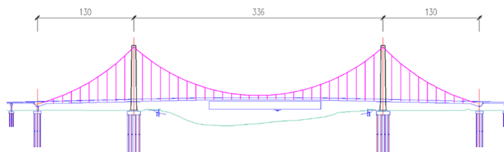
Figure 6 Self-anchored suspension bridge elevation layout diagram (unit: m)
