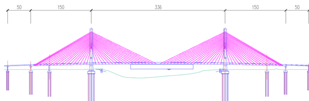
Figure 7 Cable-stayed bridge elevation layout diagram (unit: m)
