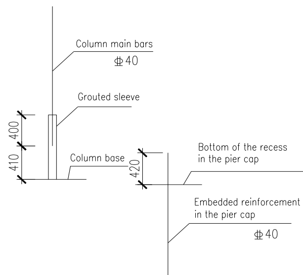
Figure 5 Reinforcement detail of grouted sleeve connections (unit: mm)
