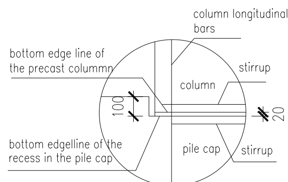
Figure 4 Prefabricated column and pile cap (unit: mm)
