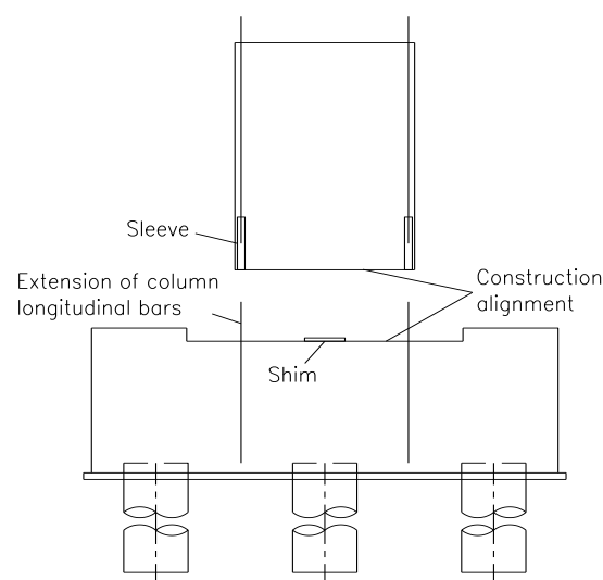
Figure 1 Schematic diagram of prefabricated assembled column construction
