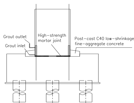
Figure 2 Schematic diagram of grouted sleeve joint construction
