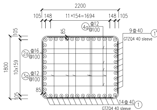
Figure 3 Reinforcement detail of the prefabricated column (unit: mm)
