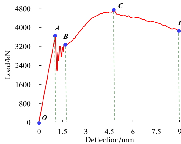
Figure 9 Mid-span load-deflection curve
