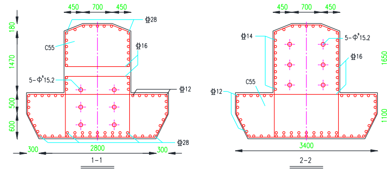
Figure 4 Cross-sectional details of the cap beam at the end (Section 1-1) and mid (Section 2-2) spans (unit: mm)
