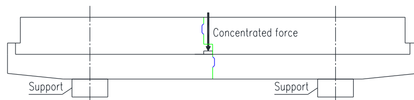
Figure 8 Schematic diagram of midspan loading
