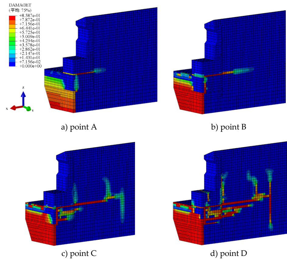
Figure 11 Tensile damage contour plot of the beam segment with an 80 mm mesh size
