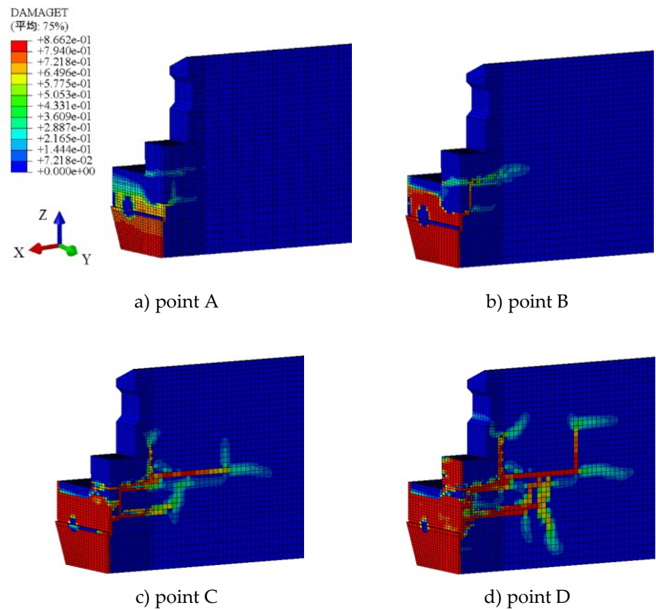
Figure 10 Tensile damage contours of the beam segment
