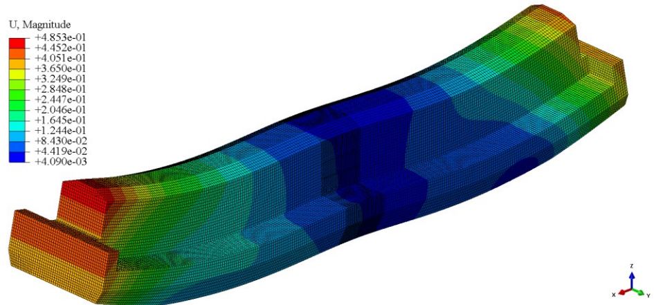
Figure 6 Concrete displacement contours of the beam segment (unit: mm)
