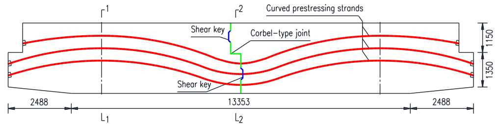
Figure 3 Half-section structural diagram of the prestressing strands in the cap beam (unit: mm)
