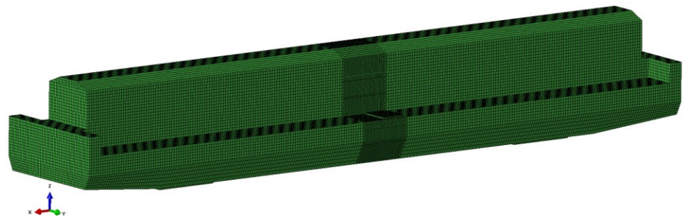
Figure 5 Finite element model
