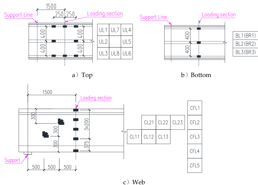
Figure 4 Concrete strain gauge layout and numbering (unit: mm)
