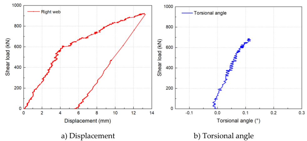
Figure 10 Load-deformation curves for the T-B side
