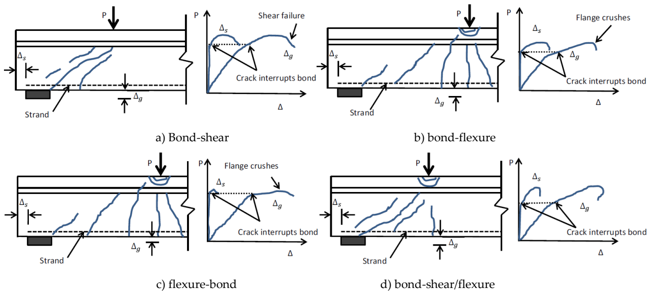
Figure 14 Typical crack pattern and structural behavior [16]
