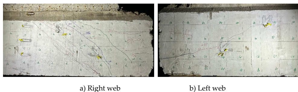
Figure 7 Crack distribution for the T-B side
