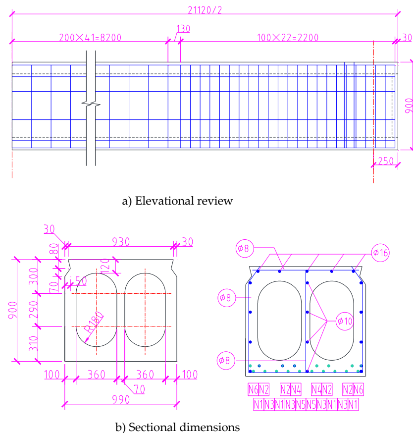
Figure 1 Construction details of the hollow core slab (unit: mm)
