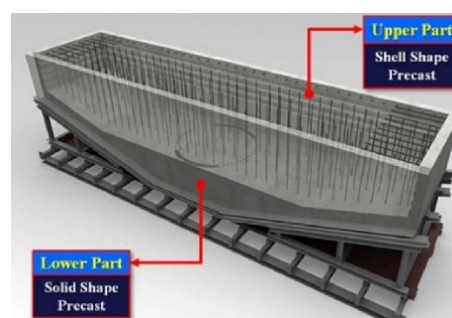
Figure 16 Prefabricated bent cap shell
