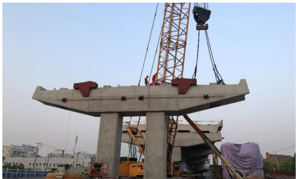
Figure 11 Construction of the Shanghai S26-5 bent cap hanging lock method
