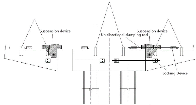
Figure 12 Lock method assembly construction diagram
