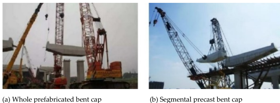
Figure 4 Fully prefabricated bent cap
